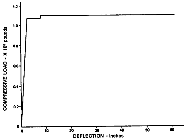
(a) NO SHEAR PLATE FAILURE
