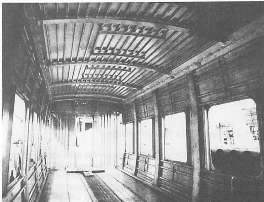
Figure 5-4 Typical Talgo HSGGT Passenger Coach Superstructure
