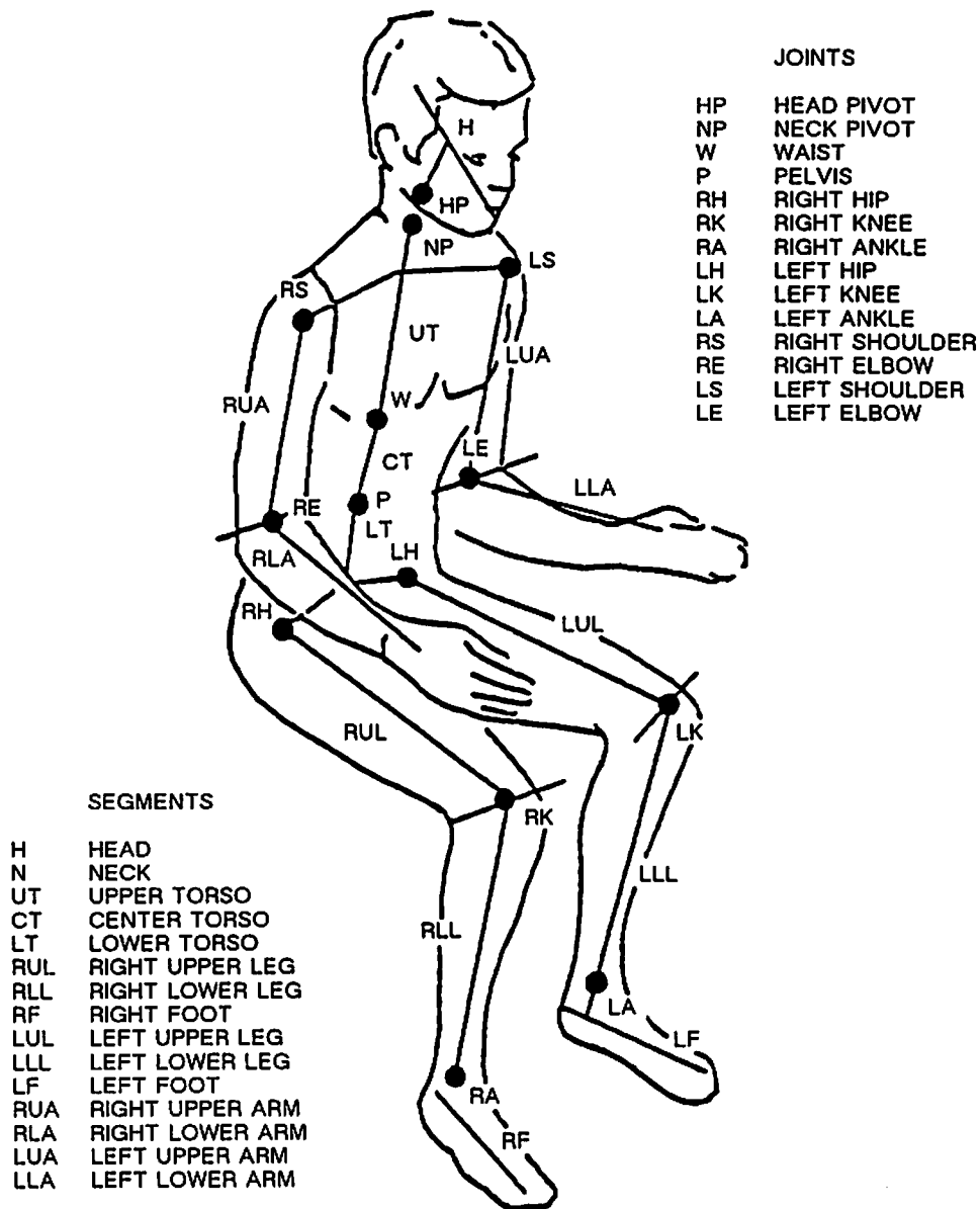
Figure 4-4 ATB Fifteen-Segment Man-Model
