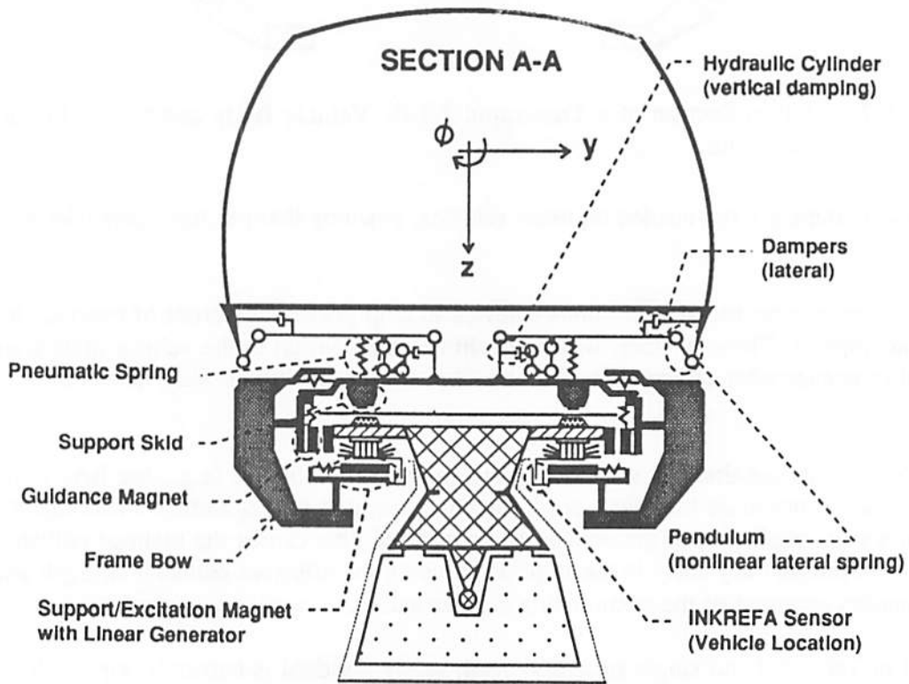
Figure 5-6 Transrapid TR-07 Suspension Systems
