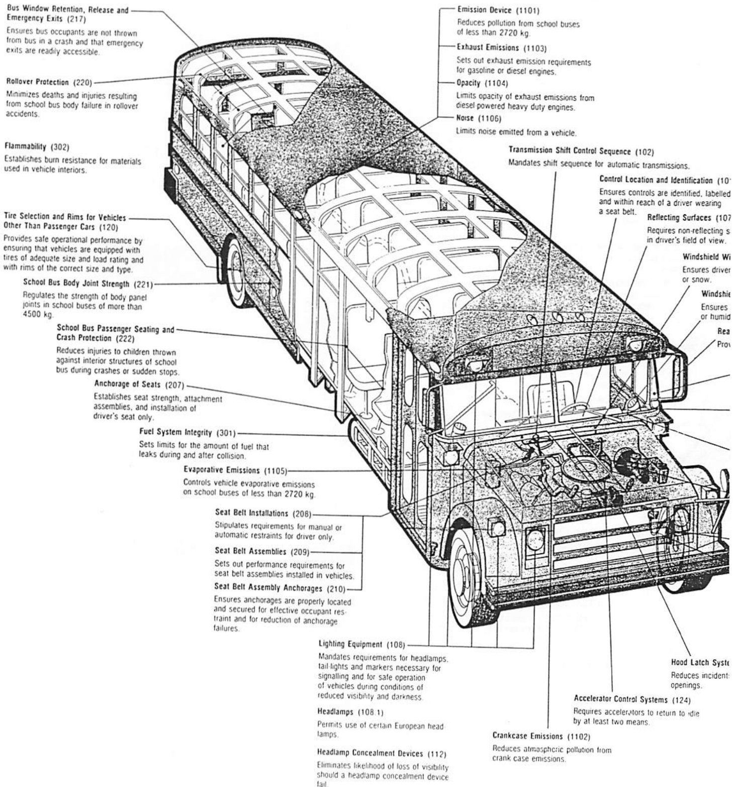
Figure 5-13 Transport Canada Motor Vehicle Safety Standards for School Buses (Illustration courtesy of Transport Canada)
