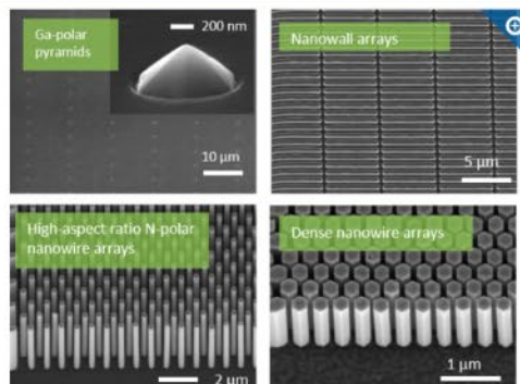
Four examples of GaN nanostructures grown with selective epitaxy by molecular beam epitaxy, illustrating different morphology for Ga-polar vs. N-polar crystals.
